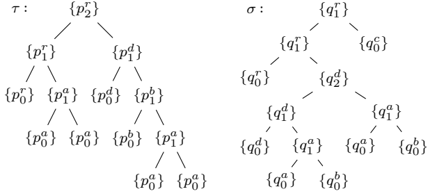
Figure 5: Synopsis trees \tau and \sigma of automata \mathcal{R} and \mathcal{T} .
