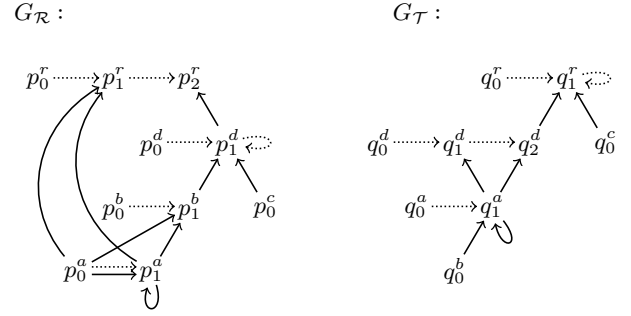
Figure 4: Transition graphs of automata \mathcal{R} and \mathcal{T} .
